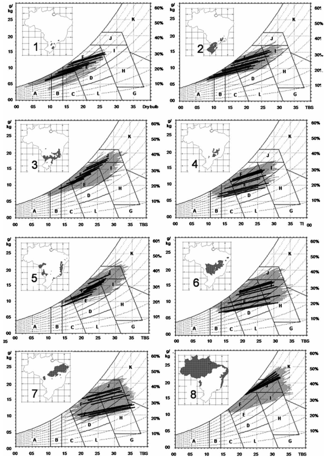
Figure 2 Bioclimatic design strategies and ventilation pattern for different zones (ABNT, NBR 15220-3, 2005).
