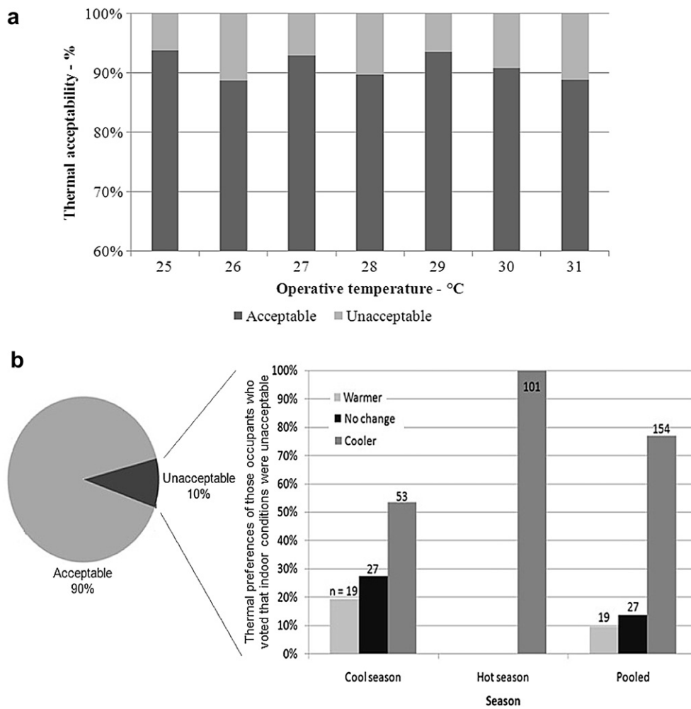
Fig. 4. (a) Thermal acceptability percentages across this study and (b) thermal preference votes separated by hot and cool seasons.
