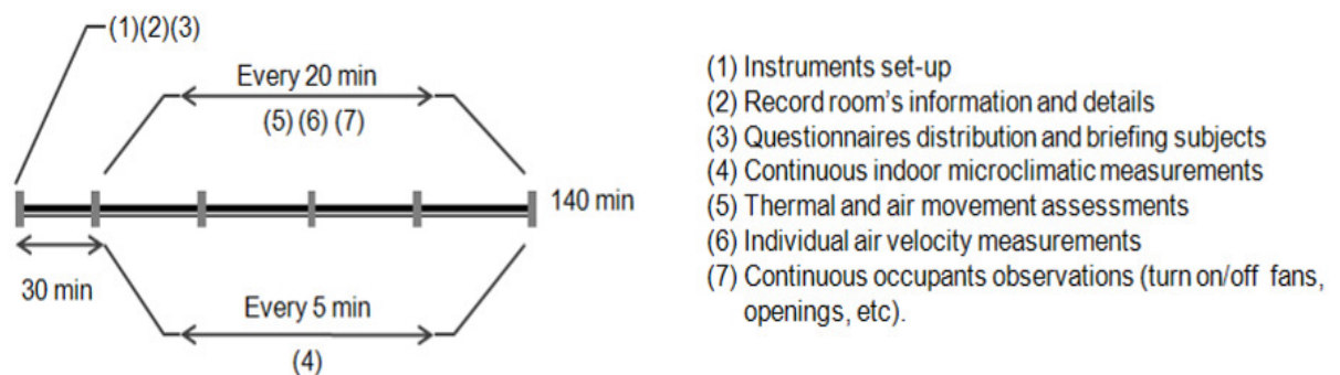
Figure 8 - Schematic representation of the measurement protocol.
