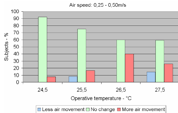
Figure 8 – Subjects’ answers for air movement preference and operative temperature: air velocity range: (a) 0 -0.25m/s and (b) 0.25 – 0.50m/s.
