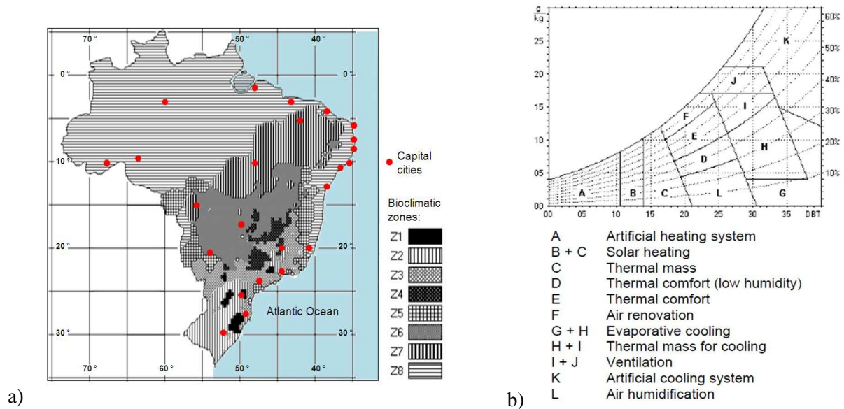
Figure 1. (a) Bioclimatic zoning and (b) bioclimatic chart (ABNT, NBR 15220-3, 2005)
