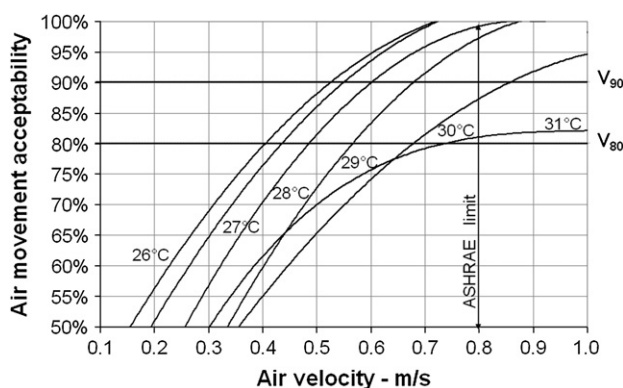
Fig. 11. Air movement acceptability and operative temperature binned by air velocity values resulted from the probit regression analysis (95% confidence levels).
