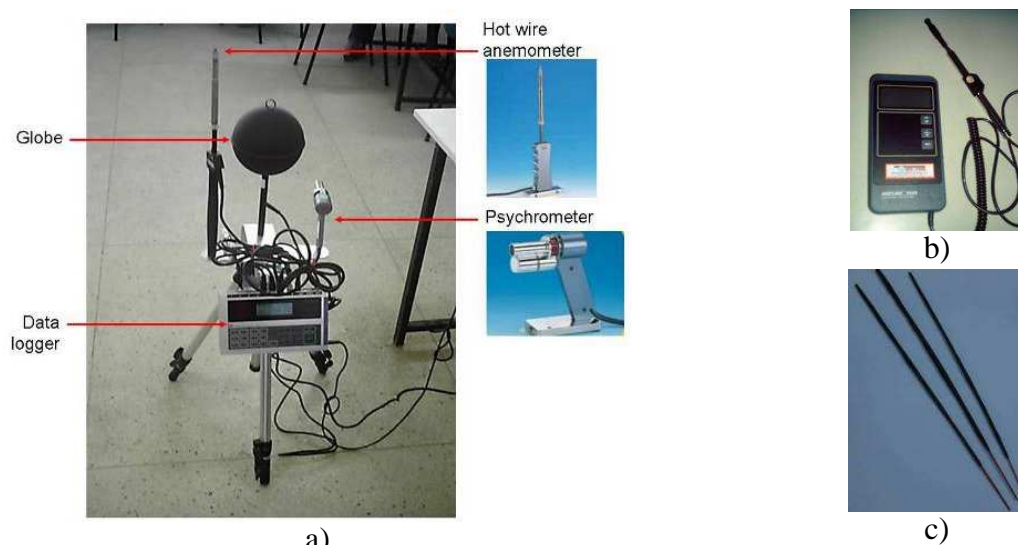
Figure 5 – Microclimatic station – Babuc (a), Hotwire anemometer (b) and Smoke stick (c)
