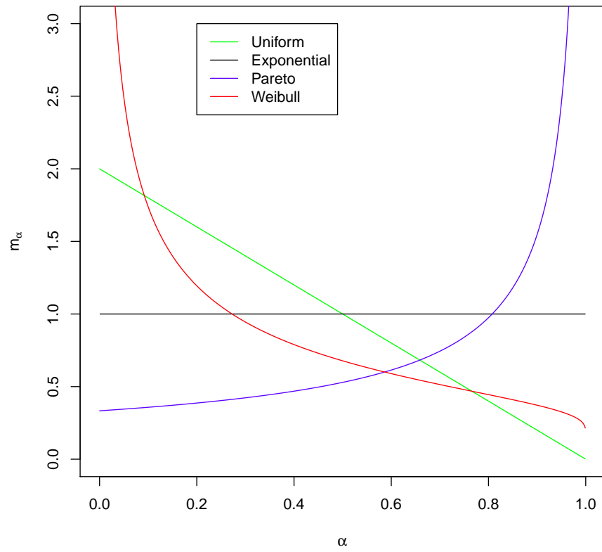
Figure 1: Mean densities for uniform ( b = 2 ), exponential ( b = 1 ), Pareto ( b = 0.5, c = 1.5 ) and Weibull ( b = 1.13, k = 2 ) distributions. All distributions have mean 1 hence the area underneath each curve is 1.
