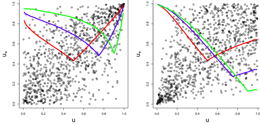
Figure 1: Left and right panels plot \theta_\alpha against \alpha for Gumbel and Clayton copulas respectively. \theta_\alpha is computed assuming a risk aversion function \phi(u) = (u > t)/(1-t) for t = 0.5 (red), 0.75 (blue) and 0.9 (green). The calculation is performed over 100 intervals of \alpha forming [0, 1] . Note how \theta_\alpha tracks local dependence (clustering along the 45^\circ line) in both copulas, apart from the kinks at \alpha = t .
