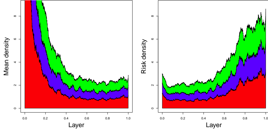
Figure 5: Left panel shows aggregate mean density and its breakdown into sub-aggregate mean densities. Right panel shows the same, for risk densities. Red, blue and green represent NASDAQ, S&P and FTSE, respectively.
