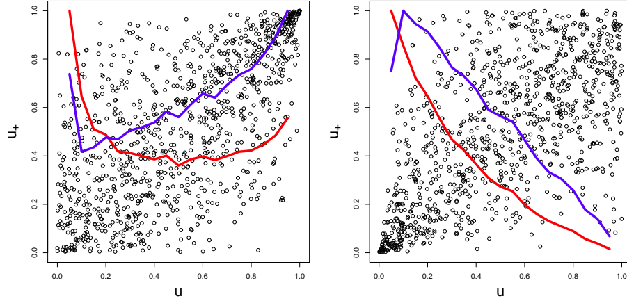
Figure 2: Left and right panels plot \gamma_\beta / \max_\beta(\gamma_\beta) against \beta for Gumbel and Clayton copulas respectively. \gamma_\beta is computed assuming x is exponential (red) and normal (blue). The calculation is performed over 20 intervals of \beta forming [0, 1] to produce smoother curves. Note how the curves trace the dependence structure of (u, u_+) represented by the scatter of points along the 45^\circ line.
