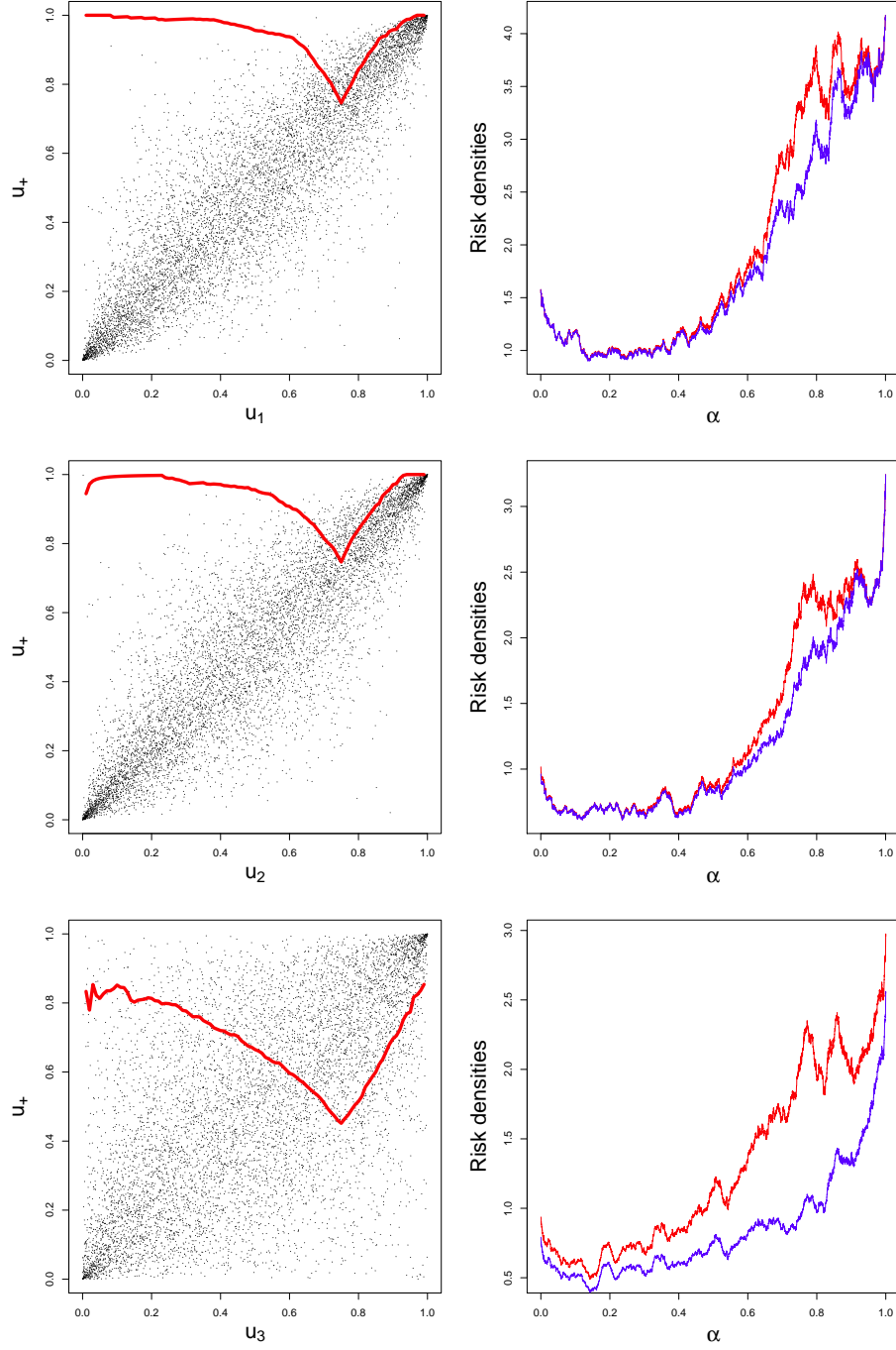
Figure 4: Left panels plot historical (u_i, u_+) and, in red, (\alpha, \theta_\alpha) . Right panels plot calculated (\alpha, r_\alpha) in red and (\alpha, \bar{r}_\alpha) in blue. Note \theta_\alpha = \bar{r}_\alpha / r_\alpha . Top, middle and bottom panels are for NASDAQ, S&P and FTSE, respectively.
