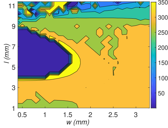
Figure 7.5: Transmission magnitude of various combinations of l and w for a constant c , ( c = 0.4 mm) at 11 GHz.
