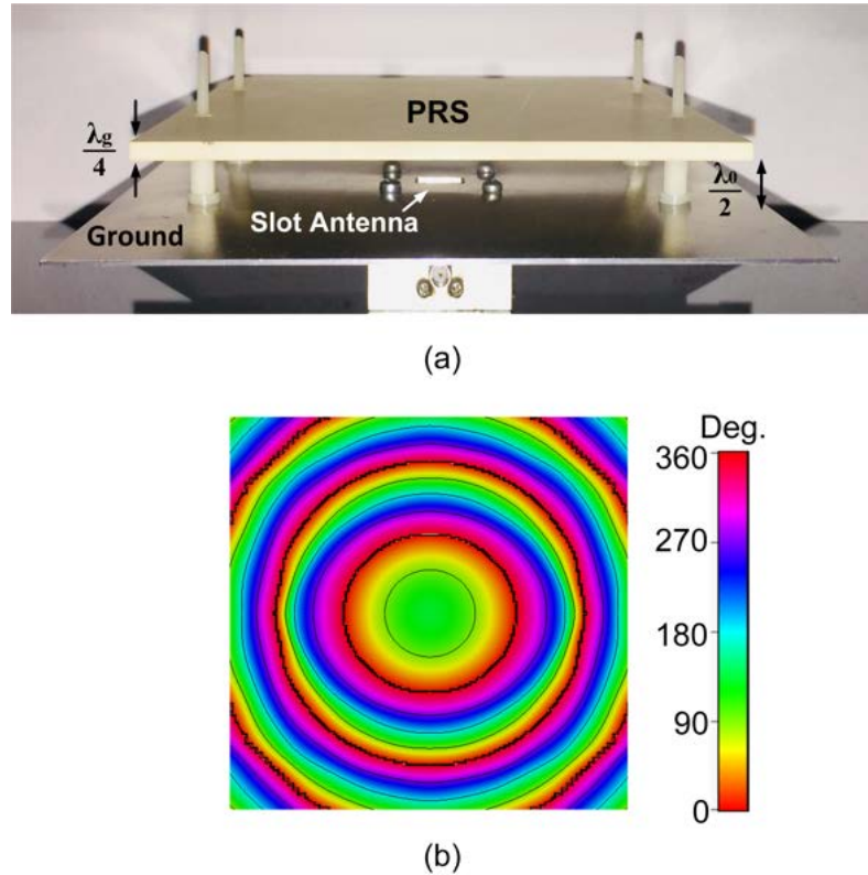
Figure 5.1: (a) A photo of the fabricated ERA with an unprinted PRS made of Rogers TMM 4. (b) 2D presentation of the phase distribution of E_y 7 mm above the antenna aperture.
